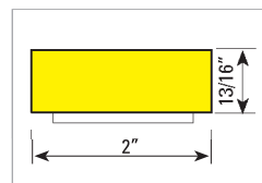
Type D: 39-3/8" x 2" x 13/16"
