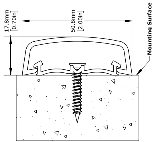
Profile View As-Installed SCALE: 1:1
