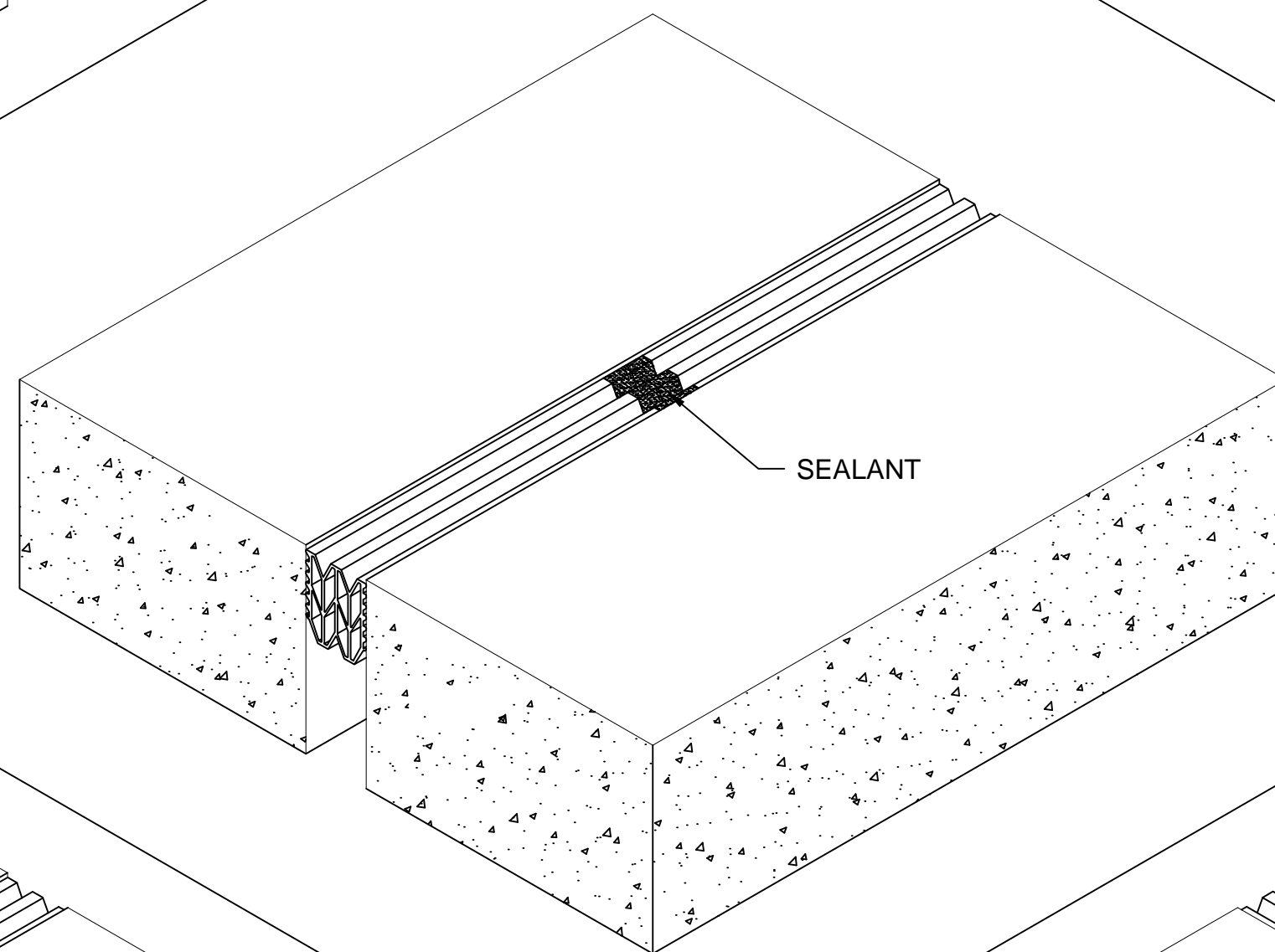
"BUTT SPLICE" TRANSITION
