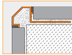
16.2 Schluter®-DESIGNBASE-SL
