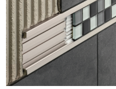
2.11 Schluter®-QUADEC-FS
