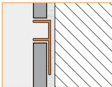
2.14 Schluter®-DECO-DE
