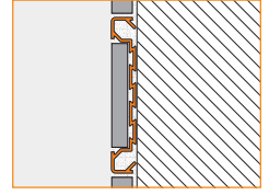
2.11 Schluter®-QUADEC-FS
