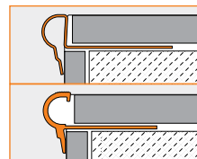
2.11 Schluter®-SCHIENE-STEP
