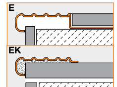
3.3 Schluter®-TREP-E/-EK
