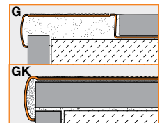
3.5 Schluter®-TREP-G/-GK
