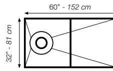
32" x 60" (81 x 152 cm) Kit with off-center drain placement
