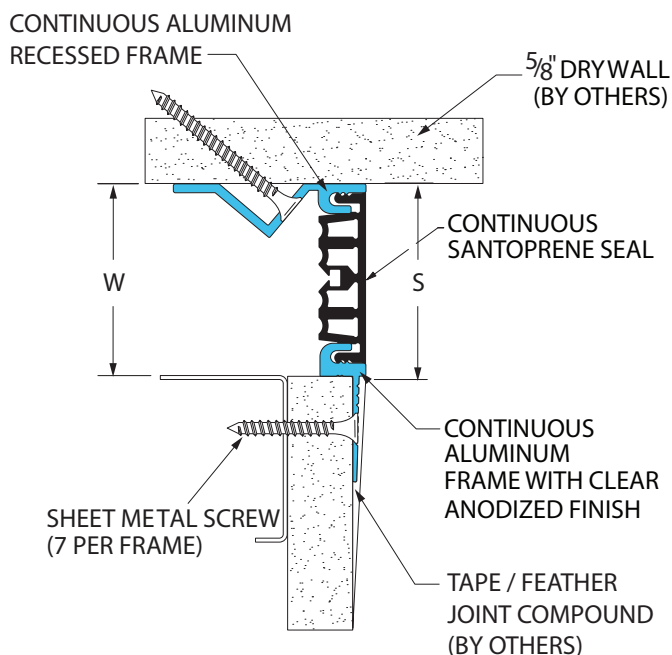
113-A09 Wall/Corner Wall/Ceiling (2" (50mm) system shown)
