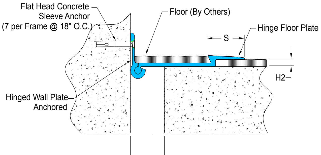
807-A02 Floor/Wall (2" (51mm) system shown)
