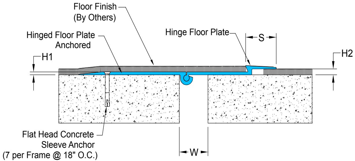
807-A01 Floor/Floor (2" (51mm) system shown)
